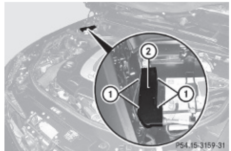
Example illustration fuse box on passenger side
