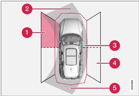
Parking sensor sectors where obstacles can be detected 119 .
