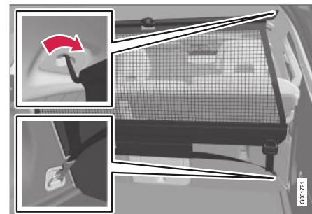
Rear mounting.
