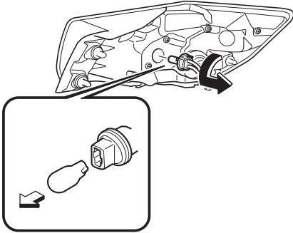
Brake lights/Taillights
