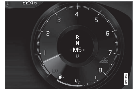
Instrument panel when the paddles are activated for shifting in manual mode, small gear selector.
