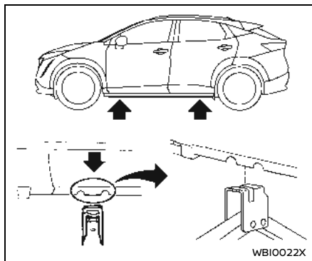
jack-up points
